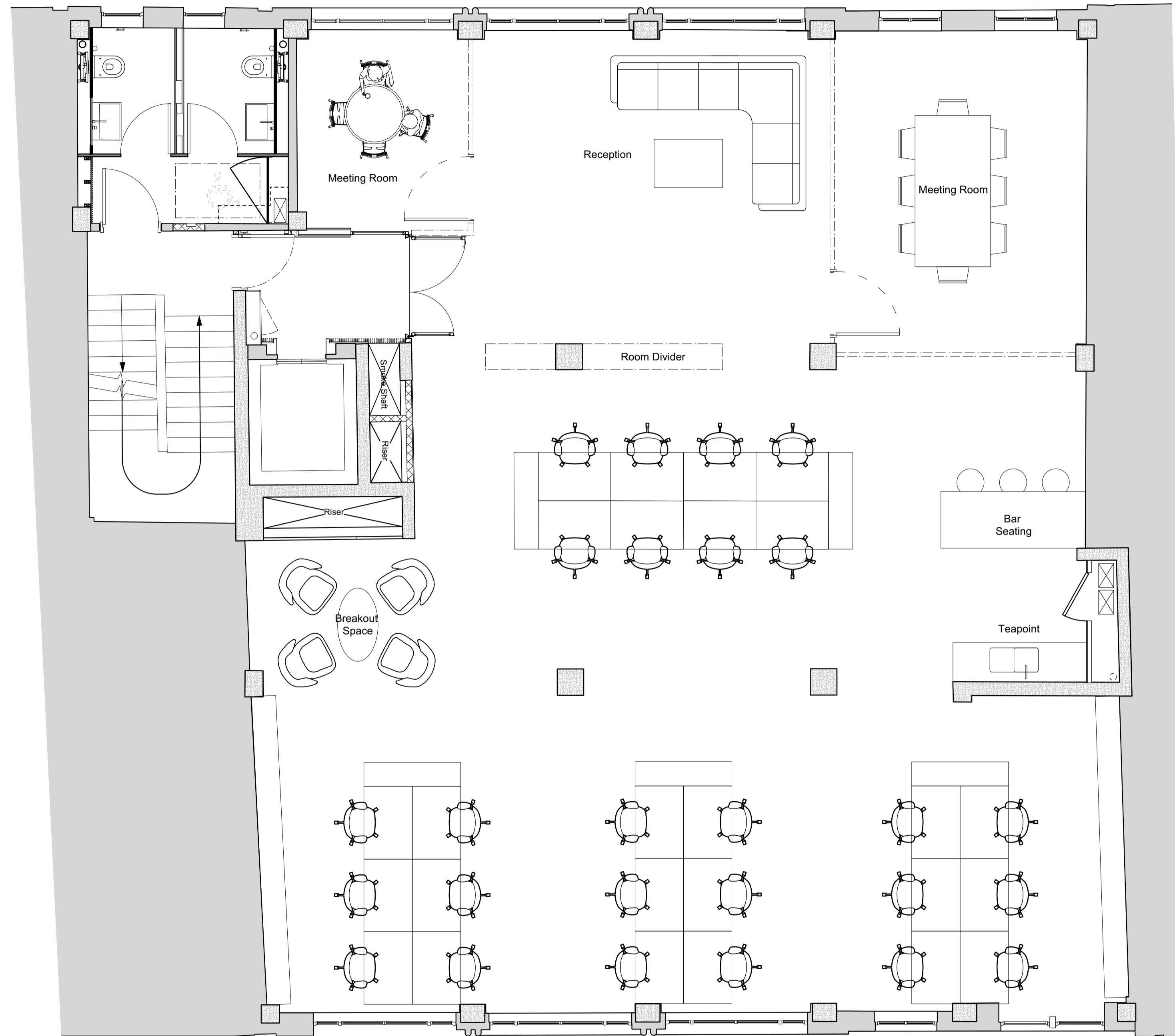
2 Typical Floor Plan - As Proposed Scale: 1:50
